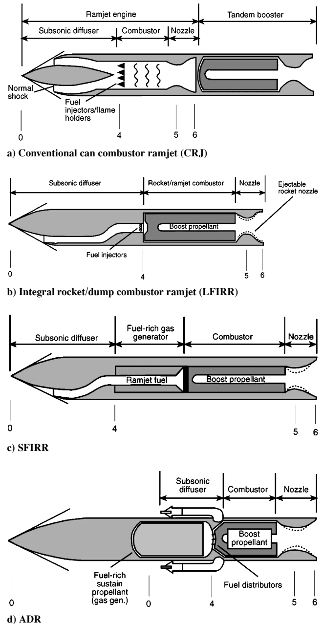
Fig. 3 Schematics of generic ramjet engines.
