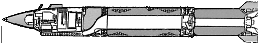
Fig. 25 U.S. SLAT flight-tested missile (1986–1992).
