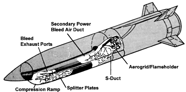
Fig. 23 U.S. ASALM flight-test vehicle (1965–1980).
