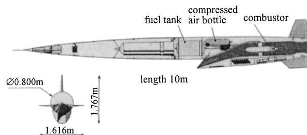
Fig. 20 French SE-X-422 flight-tested missile (1965–1967).
